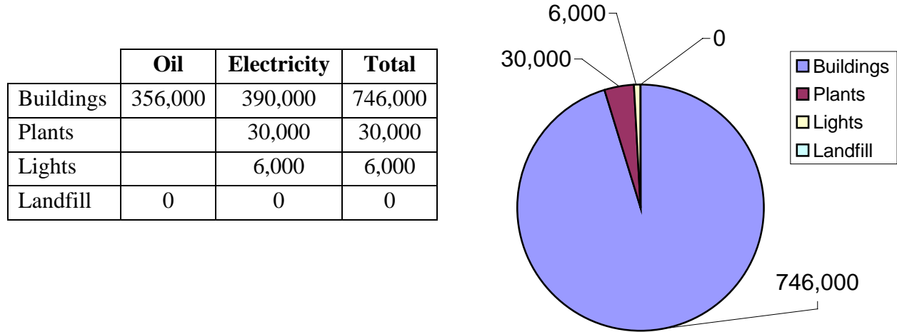
Figure 12. Municipal Emissions (tonnes CO 2 e)
